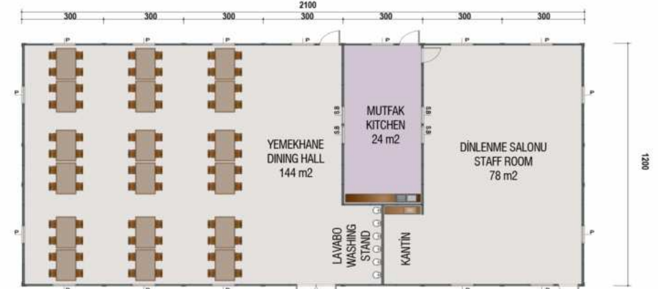
Zemin kat / Ground Floor (252m 2 )
