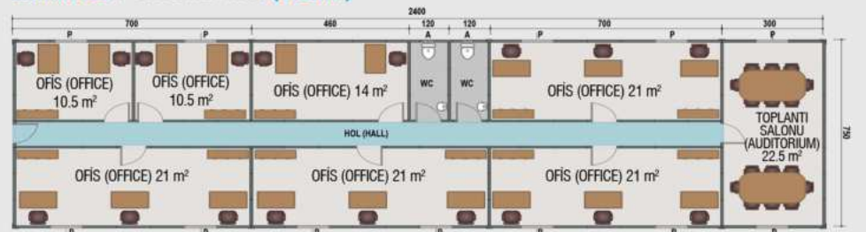
Zemin kat / Ground Floor (180m 2 )
